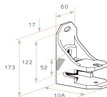
FACE FIX BRACKET (mm)
