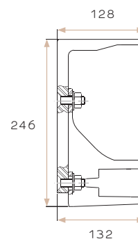
SOFFIT / TOP FIX BRACKET (mm)
